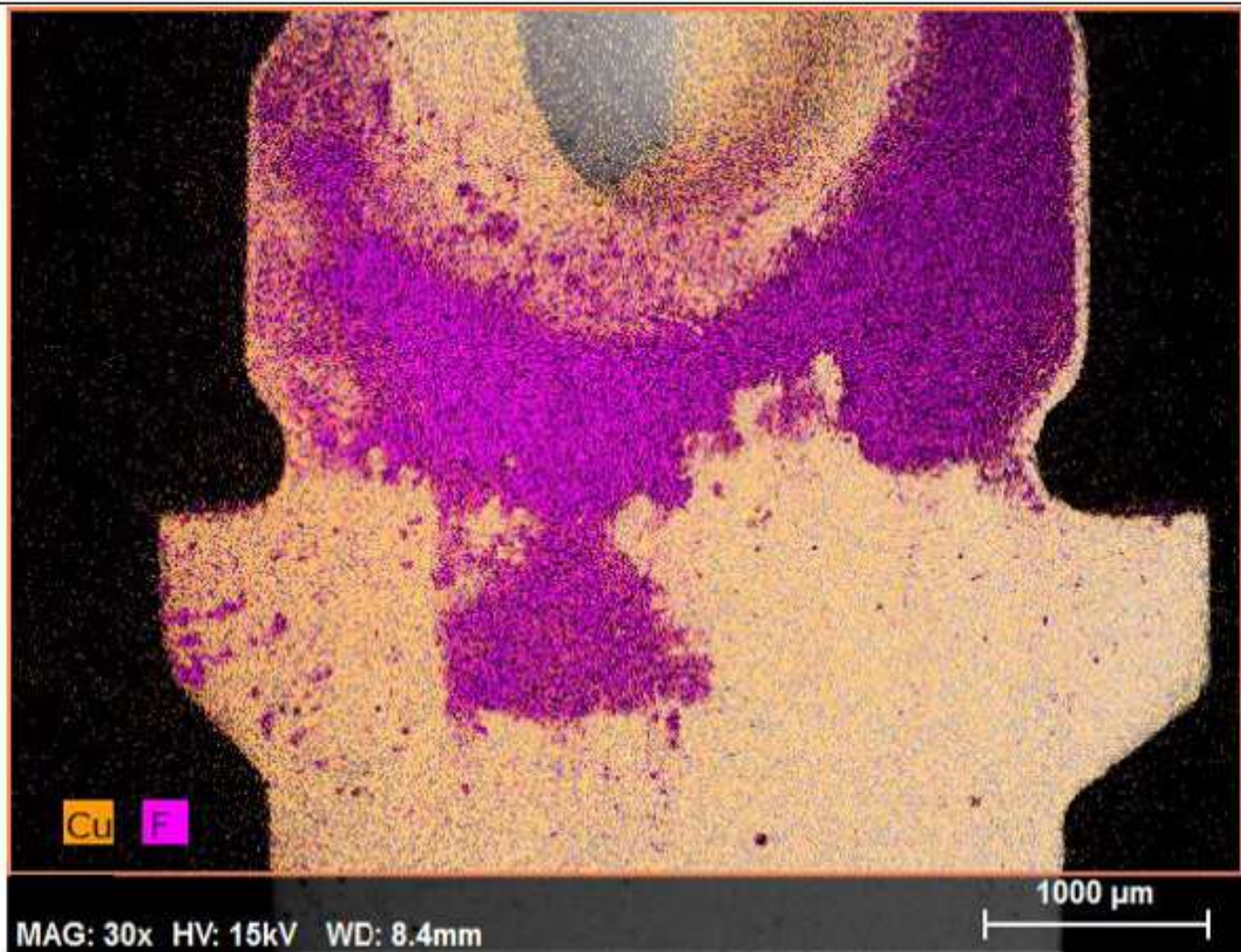
Fig. 26: EDX mapping in the middle of the copper carrier. Fluorine is clearly detected
