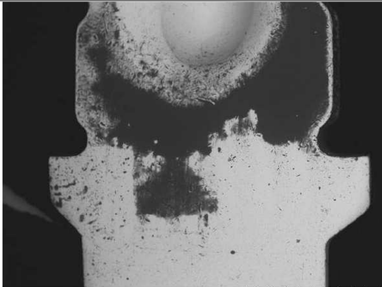
Fig.25: SEM image in the middle of the copper carrier
